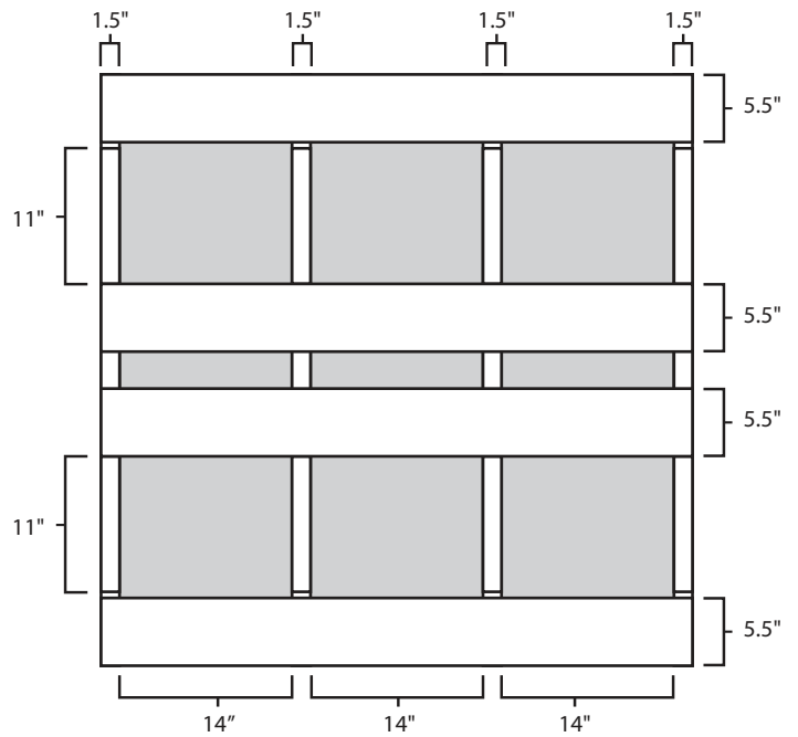
Bottom View:
